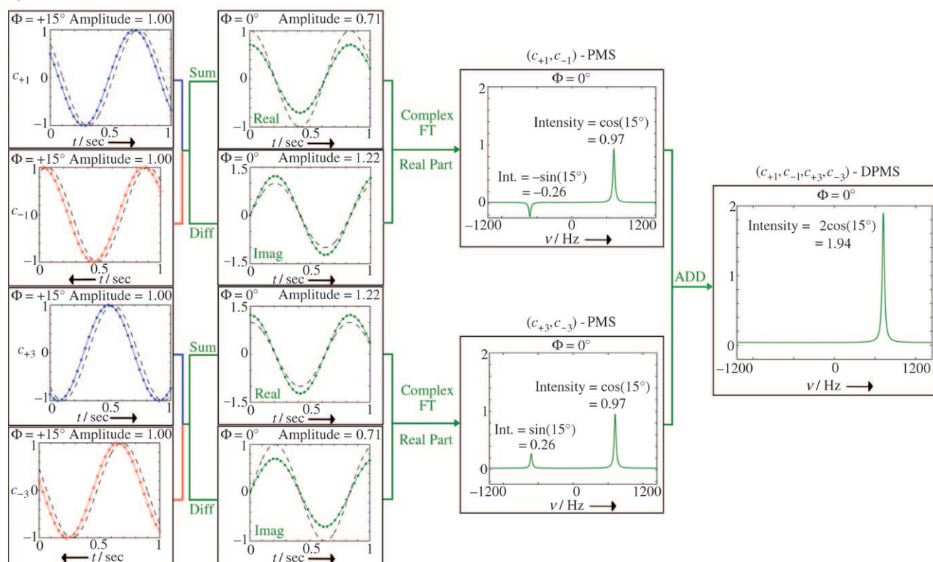
Figure 1. Clean absorption-mode NMR data acquisition a) dual "States" and b) (c_{+1}, c_{-1}, c_{+3}, c_{-3}) -dual phase shifted mirrored sampling (DPMS). The residual phase error \Phi is assumed to be 15^\circ . Forward time domain sampling and corresponding frequency domain spectra are shown in blue, backward time domain sampling and corresponding frequency domain spectra are shown in red, and linear combinations of time or frequency domain data are depicted in green. For comparison, the dashed gray lines represent time domain data of unit amplitude and \Phi = 0 . In (a) the intensities of frequency domain peaks were calculated using Eq. S68 in the Supporting Information.
